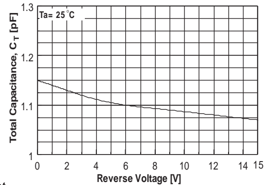
Figure 6. Total Capacitance
